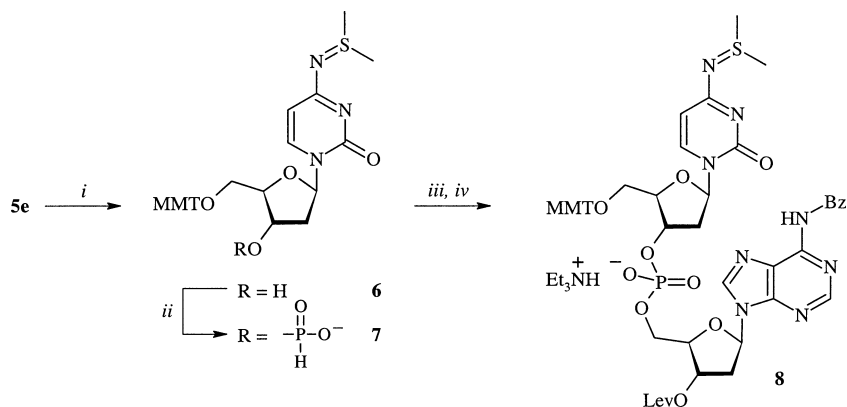
SCHEME 4 Reagents: (i) MMT-Cl/Py (ii) \text{H}_3\text{PO}_3 /Py/PivCl (iii) 3'-O-Lev-dA Bz , PivCl/Py/MeCN or OXP (iv) \text{I}_2 /Py/ \text{H}_2\text{O} .
